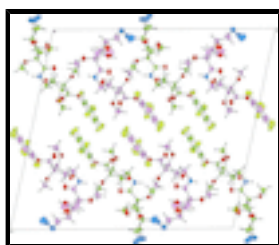
Fig. 6. The hydrogen bonded ribbons are packed side-by-side into layers. The aromatic face of one layer lies adjacent to the corresponding face of an adjacent layer.
