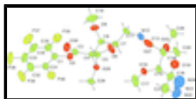
Fig. 2. The contracted molecule ( A ) in the title compound with displacement ellipsoids drawn at the 50% probability level. H atoms are shown as spheres of arbitrary radius.
